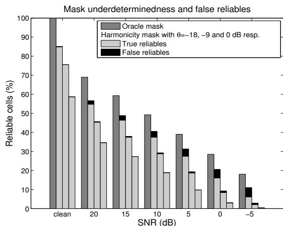
Figure 3: Percentage of reliable time-frequency cells. The figure shows results for the oracle mask as well as three threshold (0, -9 and -18) values for harmonic masks. Additionally, the figure shows the percentage of false reliables in the harmonic mask: the number of time-frequency cells labelled reliable while being unreliable according to the oracle mask.
